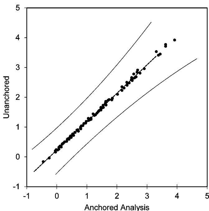
Figure 3. Person ability measures calculated using item difficulties anchored to values generated from best-fitting persons versus unanchored item difficulties.
