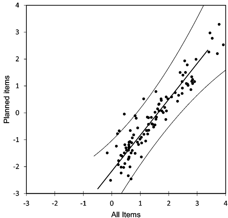
Figure 4. Person ability measures calculated from planned items versus all items. The upper and lower solid lines show the 95% confidence intervals.
