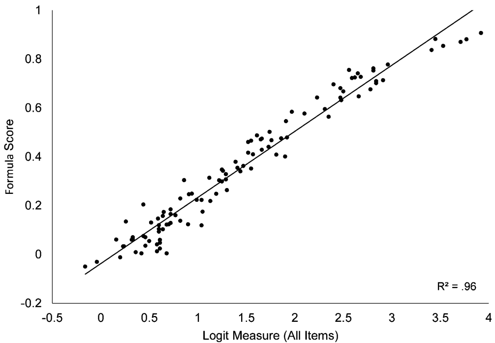
Figure 6. Formula scores versus logit measures.
