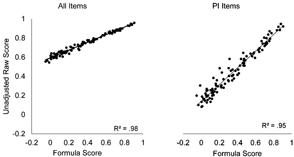
Figure 5. Raw scores versus formula scores. The left-hand panel includes all items. The right-hand panel includes only planned items. Formula scores were calculated by subtracting the proportion of incorrectly answered UI items from the proportion of correctly answered PI items.
