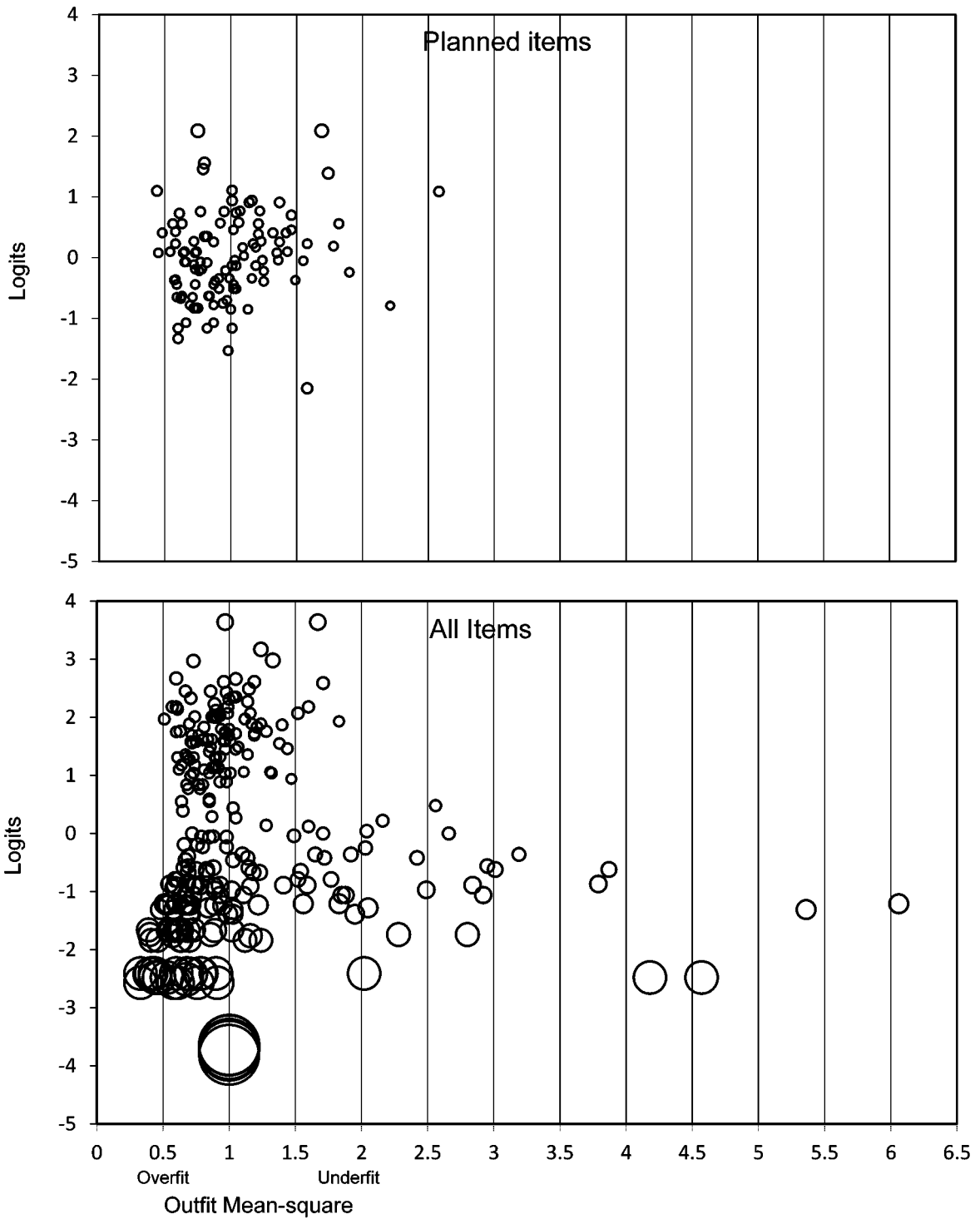
Figure 2. Item mean-square fit. The upper panel shows the planned items analyzed in isolation. The lower panel shows all items analyzed together.
