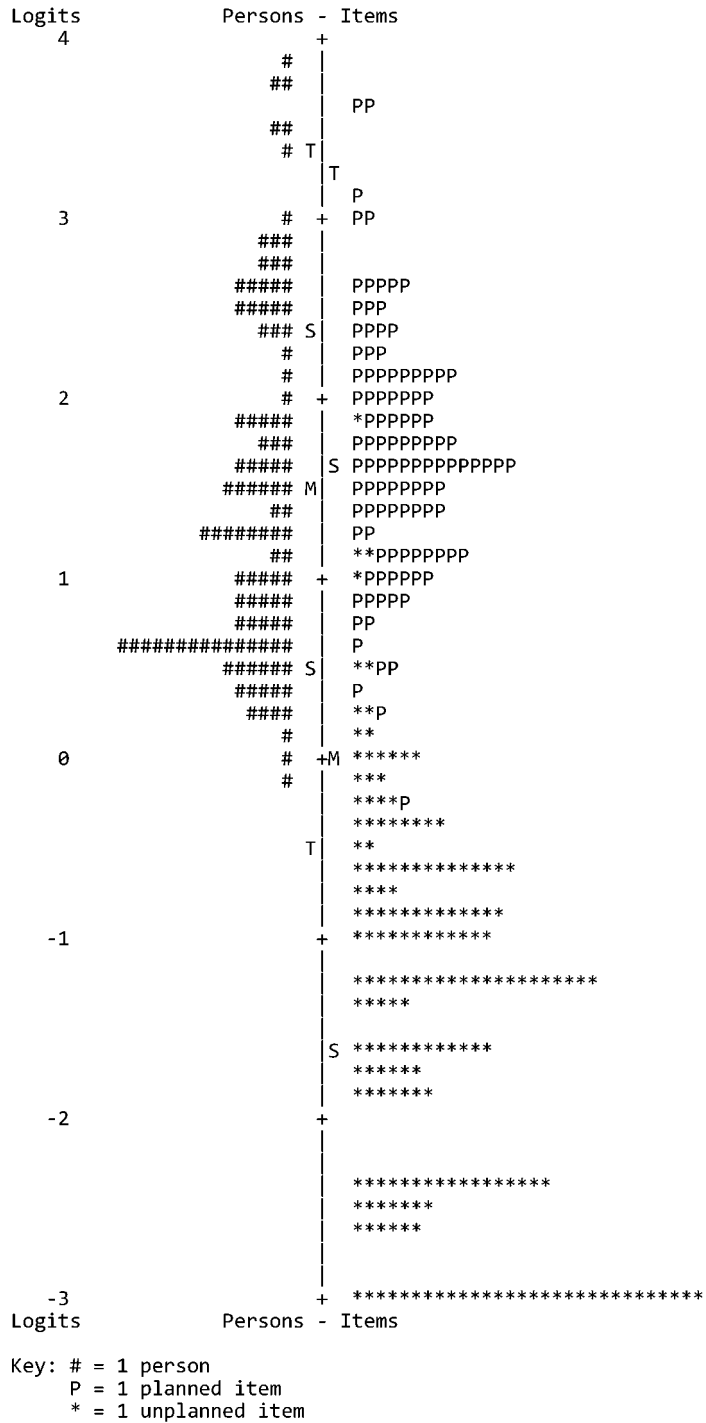
Figure 1. Person-item map. Person ability is mapped against item difficulty on a common logit scale shown on the left. A position higher on the scale indicates a higher ability person or a more difficult item.
